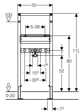
Geberit Duofix frame for washbasin, 112cm deck mounted tap
