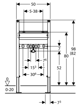
Geberit Duofix frame for washbasin, 82 - 98cm, deck mounted tap
